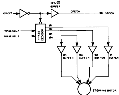
Fig. 7-34. Block diagram of track select circuit, Model 1541.
